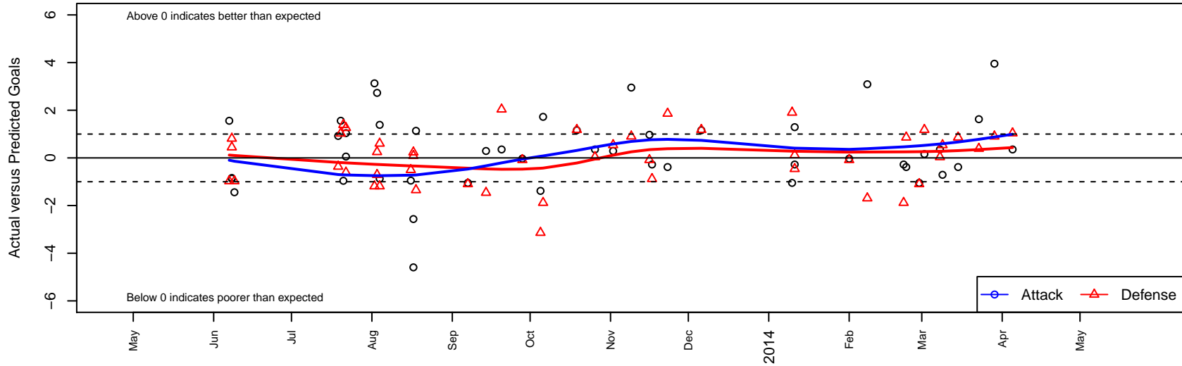
Crossfire Premier B G02 Dots are actual minus expected GF (blue circles) and GA (red triangles). Blue line is smoothed change in attack strength. Red is smoothed change in defense strength.
